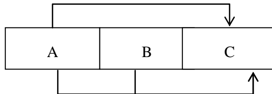
Figure 10.8 Non-key attribute C is partially dependent on the key {A,B}
