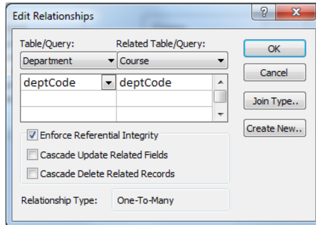
Figure 6.31 Join properties
