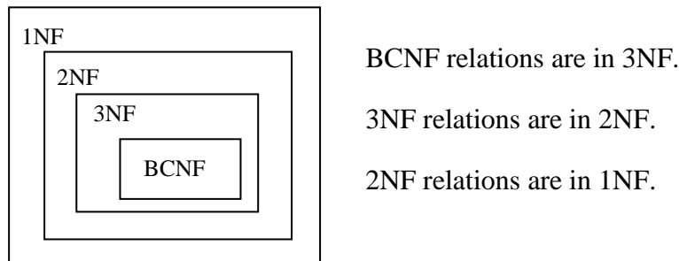
Figure 10.1 Normal forms
