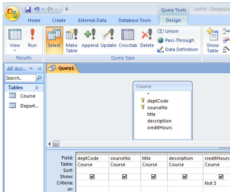
Figure 6.3 Using NOT
