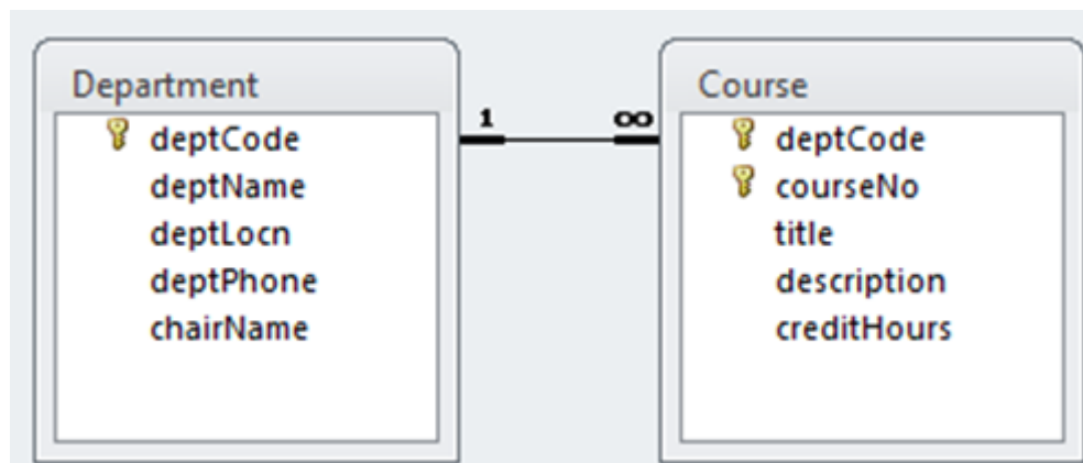
Figure 6.30 Standard equi-join
