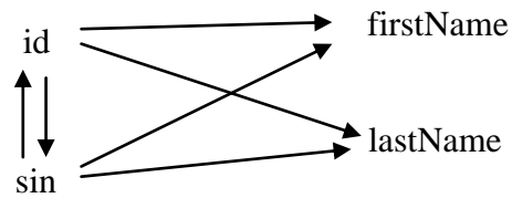
Figure 10.6 FDs that must be present given the ERD in figure 10.5
