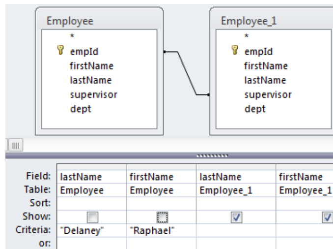
Figure 6.40 Self-join
