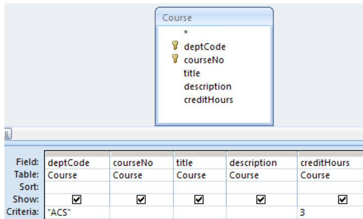
Figure 6.1 Two expressions that are ANDed
