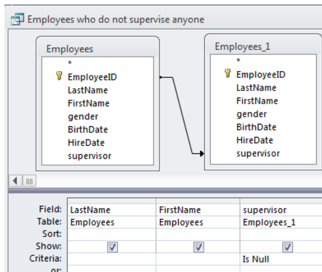
Figure 6.41 Anti-join
