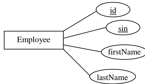
Figure 10.5 ERD for an Employee entity type
