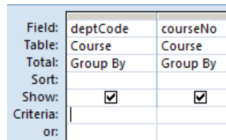
Figure 6.19 Step 2: Total line is added to the grid
