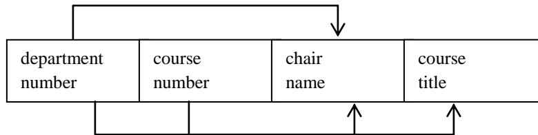
Figure 10.7 Chair name is partially dependent on the PK
