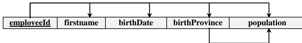
Figure 10.16 A non-3NF relation (transitive dependency shown)
